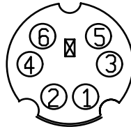
6-pol. Mini-DIN Buchse,
